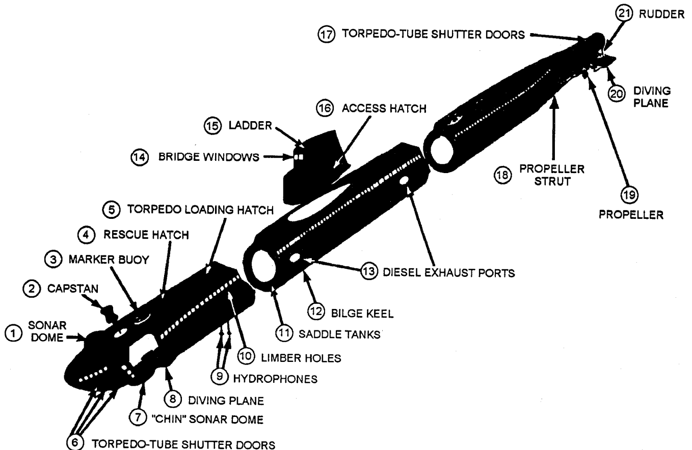
Figure 6-23.—Older submarine.
